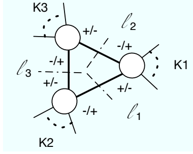
Figure 6: The triple-cut contribution the amplitude.
