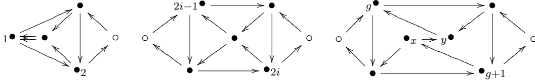
FIGURE 3. Three building blocks for a quiver in \mathcal{Q}_{g,1} . Gluing points are marked with \circ .
