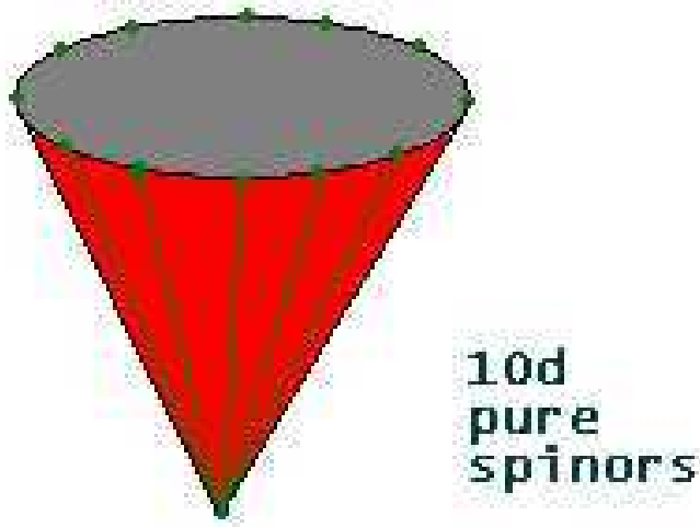
Fig. 1: The space of pure spinors in ten dimensions and the fixed lines entering (3.25)
