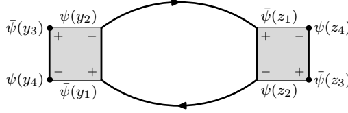
Figure 4: A UV logarithmically divergent planar diagram contributing to the \beta -functions, related to the amplitude (3.14).
