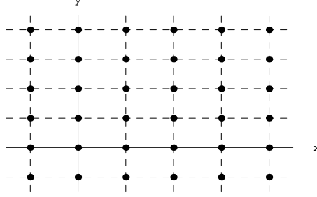
FIGURE 1. A periodic graph
