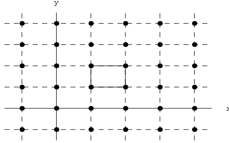
FIGURE 2. A cycle with |\Gamma_C| = 1
