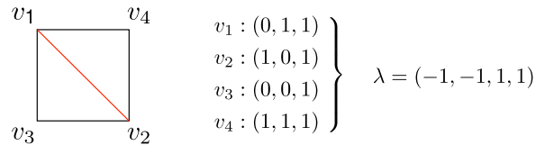
Figure 4: The 2-cone \sigma corresponds to the relation \bar{\lambda} among 1-cones.
