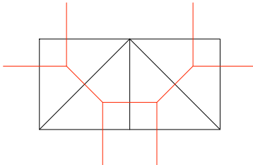
Figure 1: Example of a box triangulation, corresponding to a 3 dimensional toric fan. The diagram in red is the dual web diagram. Vertices of the triangulations (faces of the web diagram) correspond to 1-cones, edges correspond to 2-cones, and faces (vertices of the dual) correspond to 3-cones.
