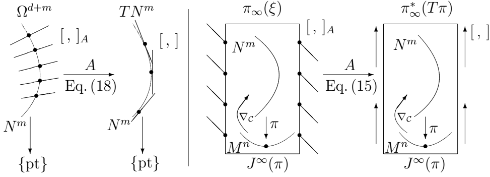
FIGURE 3. From Lie algebroids (\xi, A, [\cdot, \cdot]_A) to variational Lie algebroids (\pi_\infty^*(\xi), A, [\cdot, \cdot]_A) .
