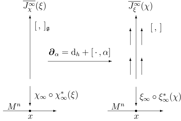
FIGURE 1. Non-Abelian variational Lie algebroid.
