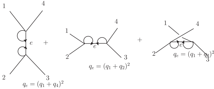
FIGURE 2. Summing over orientations, a twice-marked edge gives a contribution proportional to the sum of its external propagators x_i = q_i^2 (in the massive case, massive vertices v(0) guarantee the same result for x_i = q_i^2 - m^2 ).
