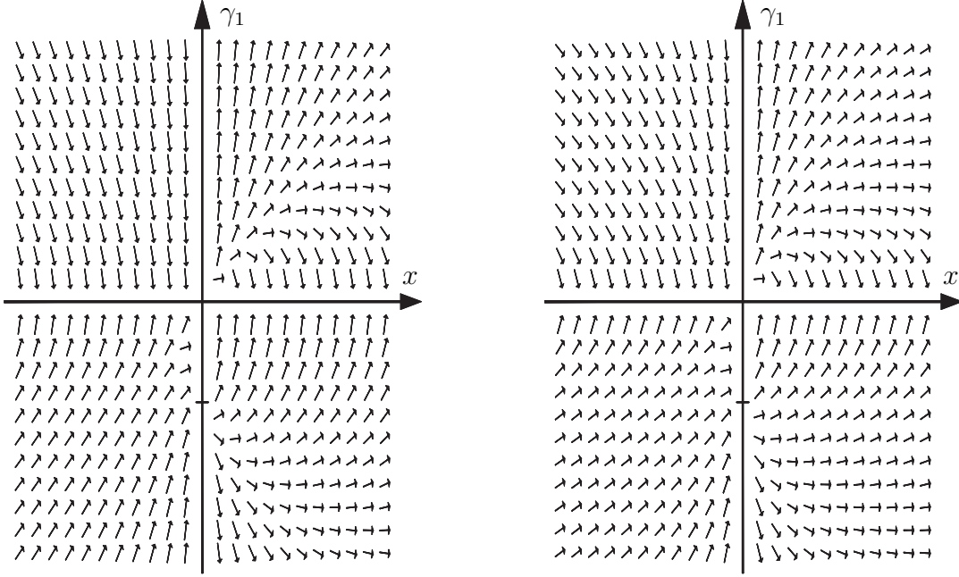
Figure 1: Direction fields for P(x) = x , s = 1 on left panel, s = 2 on right panel. Note how the two pictures look similar; yet, as will be shown, the s = 1 case admits global positive solutions, and s = 2 does not.
