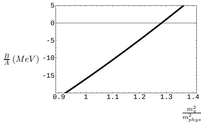
Figure 5: The binding energy, B , per nucleon in nuclear matter as a function of the pion mass.
