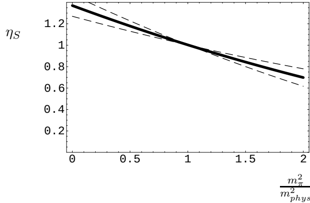
Figure 2: The value of the scalar strength \eta_S as a function of the pion mass.
