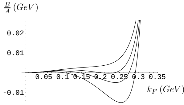
Figure 4: The binding energy, B , per nucleon in nuclear matter as a function of the Fermi momentum for various values of the scalar strength G_S . From bottom to top in the figure, the values of -G_S are (362, 340, 328, 315) \text{GeV}^{-2}
