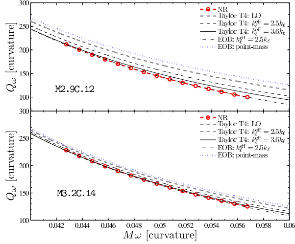
FIG. 2: The same as Fig. 1 but when using the Taylor-T4 approximant either at LO (thick dashed line) or at NLO with different amplification factors (solid and dashed lines). Also shown as a reference is the EOB Q_\omega curve at NLO with \kappa_\ell^{\text{eff}} = 2.5\kappa_\ell (dot-dashed line).
