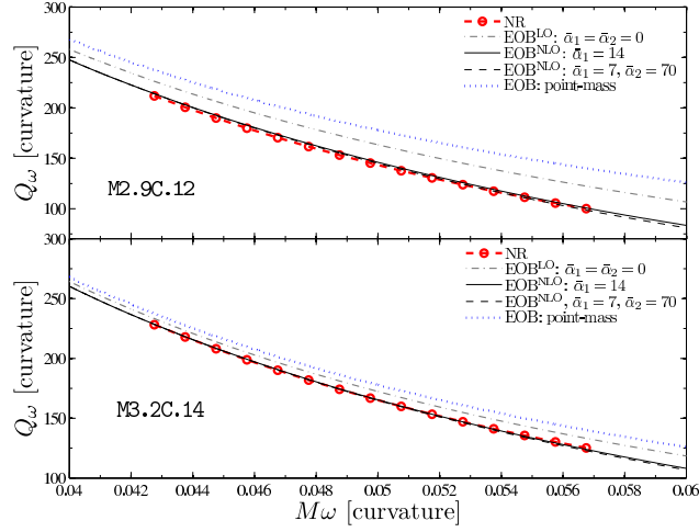
FIG. 1: Comparison of the AR curves for Q_\omega at NLO for different choices of the parameters (solid, dashed lines) with the corresponding NR ones (dashed lines with open circles) for the two binaries considered. Also shown are the Q_\omega curves for the LO term (dot-dashed line) and when tidal effects are ignored (dotted line).
