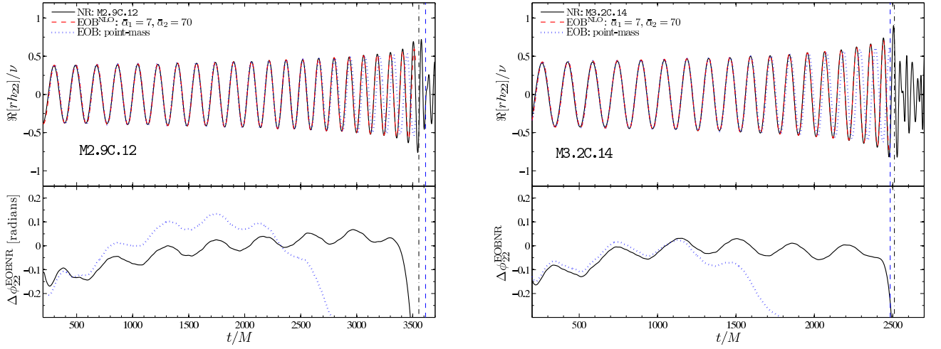
FIG. 3: Comparison between NR and AR phasing for the M2.9C.12 (left panels) and M3.2C.14 (right panels) binaries. The top panels show the real parts of the h_{22} waveforms, while the bottom panels show the corresponding phase differences. Note the excellent agreement almost up to the time of merger (vertical dashed and dot-dashed lines) and the very large errors when tidal effects are neglected (dotted line).
