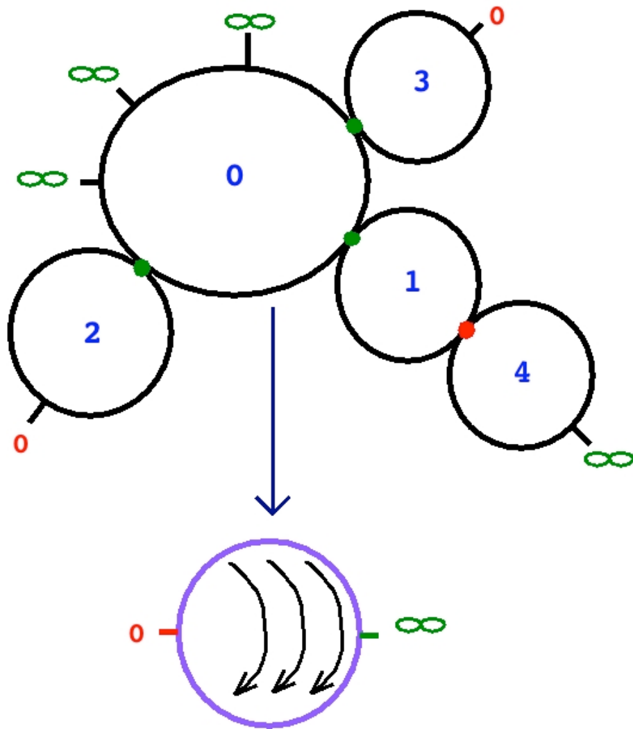
Fig.2 An example of a C^* -invariant stable map
