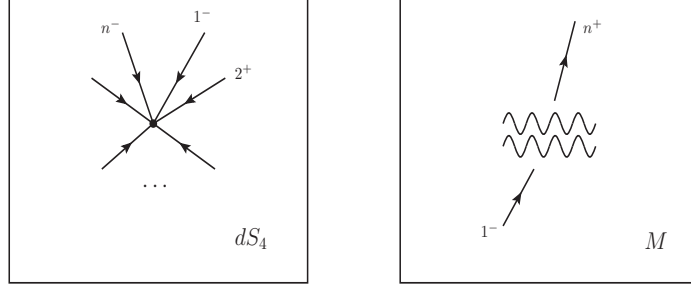
Figure 3. Geometric picture of MHV graviton scattering
