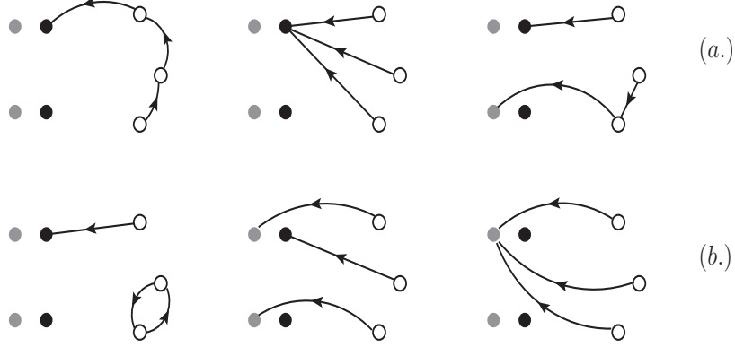
Figure 7. Some diagrams for the 5-point amplitude which have a non-vanishing (a.), or excluded/vanishing (b.) contribution.
