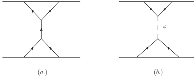
Figure 4. In minimal \mathcal{N} = 4 CSG, external gravitons only couple to other gravitons in the bulk (a.); in the non-minimal model they can couple to the scalar \varphi (b.).
