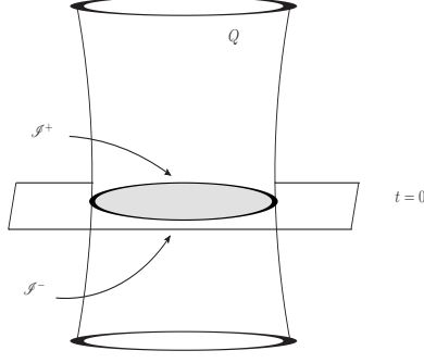
Figure 1. De Sitter space as the quadric Q \subset \mathbb{RP}^5 and the identification of infinity.
