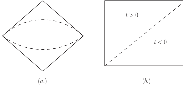
Figure 2. De Sitter space on the affine Minkowski slicing (a.), and the traditional Poincaré slicing (b.)
