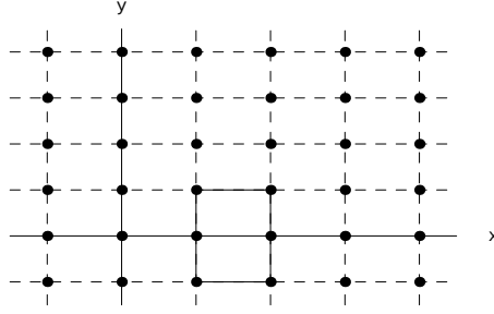
FIGURE 3. A cycle with |\Gamma_C| = 2
