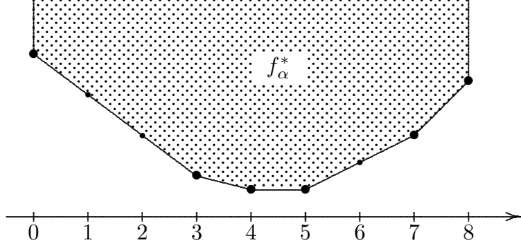
Figure 2: Typical set f_\alpha^* , with n_\alpha = 8 , r = 5 , and (k_0, \dots, k_5) = (0, 3, 4, 5, 7, 8) .
