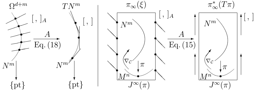
FIGURE 3. From Lie algebroids (\xi, A, [\cdot, \cdot]_A) to variational Lie algebroids (\pi_\infty^*(\xi), A, [\cdot, \cdot]_A) .
