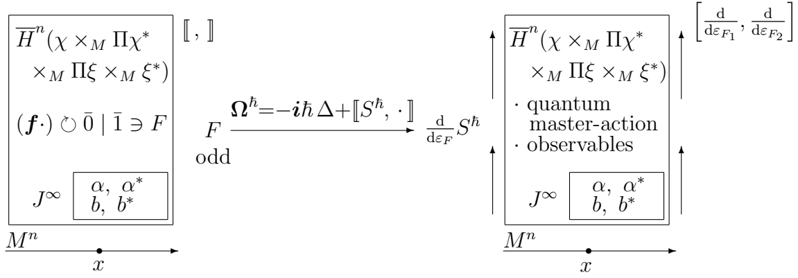
FIGURE 2. The next generation of Lie algebroids: gauge automorphisms of the (quantum) BV-cohomology.
