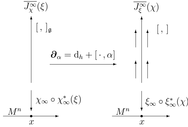
FIGURE 1. Non-Abelian variational Lie algebroid.
