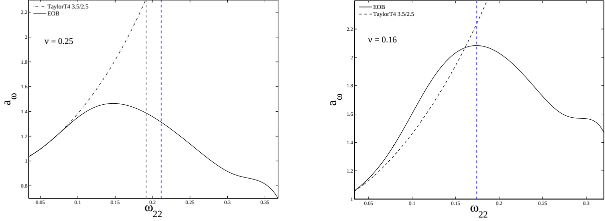
FIG. 11: Comparison between phase acceleration curves a_\omega of EOB (solid line) and TaylorT4 (dash-dot line) for \nu = 0.25 (left panel) and \nu = 0.16 (right panel). The rightmost dashed vertical line indicates the location of the EOB adiabatic LSO. The leftmost vertical line on the left panel indicates the EOB GW frequency corresponding to the instant when T4 blows up.
