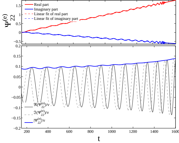
FIG. 9: Same as Fig. 8 except that the integration and the linear fit have been done starting at time t \sim 150 , i.e. at the beginning of the inspiral signal. Note the oscillations in the modulus of the bottom panel, and the fact that the linear drifts (visible in the upper panel) are much larger than in Fig. 8.
