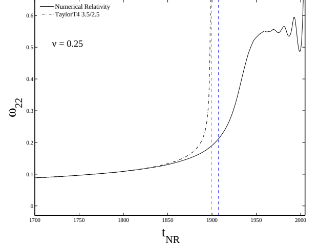
FIG. 10: Numerical relativity (Jena) and TaylorT4: comparison between the instantaneous gravitational wave frequencies for the equal mass case ( \nu = 0.25 ).
