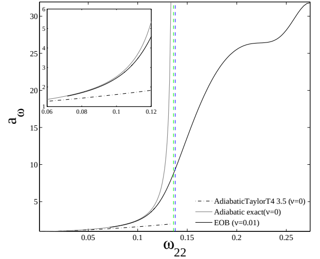
FIG. 12: This figure (done for \nu \ll 1 ) illustrates, in particular, the fact that the domain of validity of TaylorT4 when \nu \lesssim 0.16 reduces to the “normal” 3.5 PN one, namely \omega \lesssim 0.06 .
