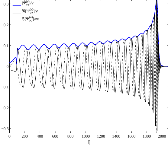
FIG. 7: Computation of the Zerilli normalized metric waveform \Psi_{22}^{(e)} from r\psi_4^{22} via two backward time integrations starting with zero integration constants at the final time. The data refer to the 1:1 mass ratio ( \nu = 0.25 ) numerical simulation. Unphysical oscillations in the modulus are quite visible at early times.
