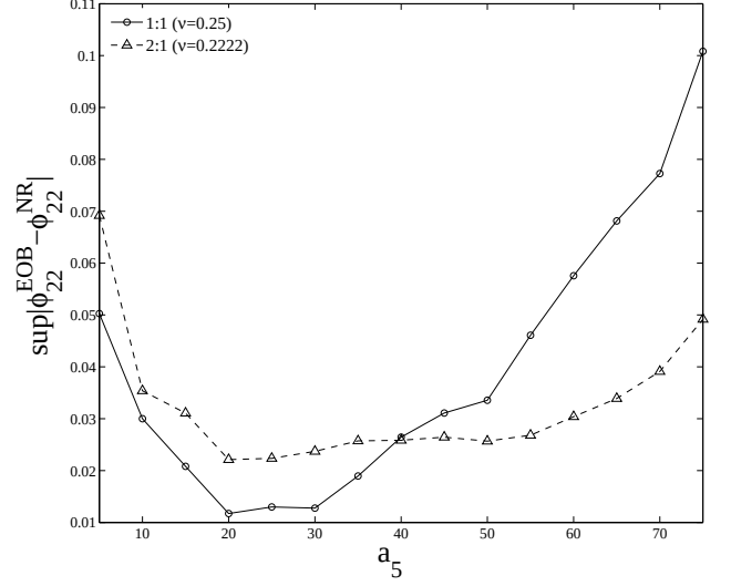
FIG. 3: L_\infty norm of the EOB-NR late-inspiral ( [t_L, t_R] ) phase difference, as a function of a_5 for \nu = 0.25 (1:1 mass ratio) and \nu \simeq 0.2222 (2:1 mass ratio). NR refers to results Jena coalescence simulations reported here.
