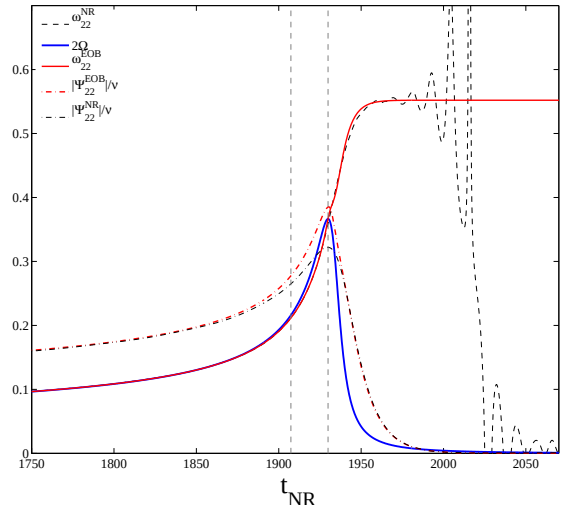
FIG. 5: Comparison between EOB and NR instantaneous gravitational wave frequencies (and moduli) for the equal mass case, \nu = 0.25 . Here, as in Fig 6, NR refers to the Jena coalescence simulation. The two dashed vertical lines refer, respectively, to the EOB adiabatic LSO and to the “EOB light-ring”.
