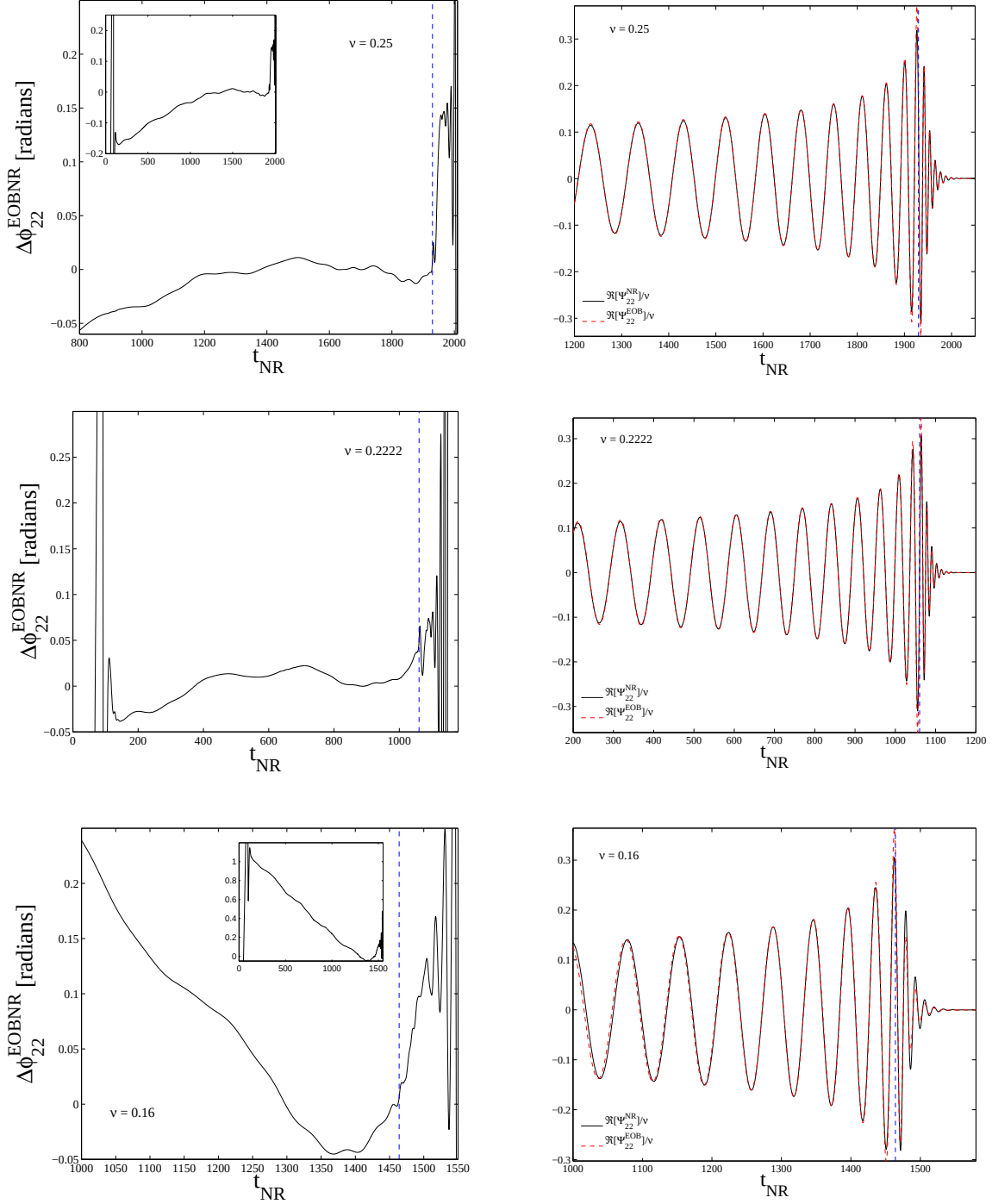
FIG. 4: Comparison between NR and EOB waveforms for \nu = 0.25 (top), \nu = 0.2222 (middle) and \nu = 0.16 (bottom). The left panels depict the EOB-NR phase difference; the right panels show the real part of the metric waveforms. Here, NR refers to the full results of Jena coalescence simulations, from early-inspiral to ringdown, by contrast to the L_\infty norm of Fig. 3 which concerned a late inspiral stage [t_L, t_R] . The dashed vertical lines in the figures mark the location of the “EOB light-ring”.
