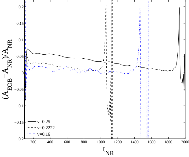
FIG. 6: Fractional EOB-NR differences in the gravitational wave (metric) amplitudes, A \equiv |\Psi_{22}| , versus NR time for different mass ratios.
