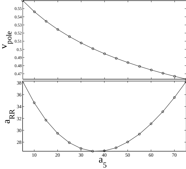
FIG. 1: Functional relationships linking v_{\text{pole}} and \bar{a}_{\text{RR}} to a_5 obtained by imposing the two constraints (15)-(16) based on published Caltech-Cornell inspiral waveform data.
