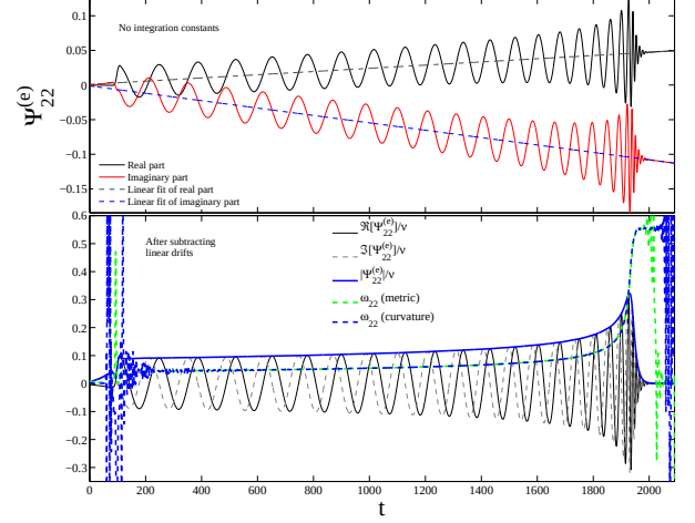
FIG. 8: Computation of the metric waveform \Psi_{22}^{(e)} from r\psi_4^{22} via two time integrations starting at t = 0 . The upper panel has zero integration constants and exhibits clear linear drifts \alpha t + \beta . The bottom panel shows the result of subtracting the linear drift of the waveform obtained by fitting the upper panel over the entire time interval starting at t = 0 .
