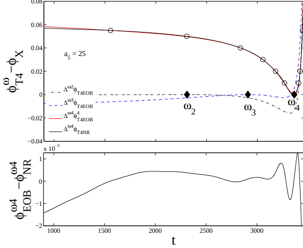
FIG. 2: Top panel: near-perfect agreement between T4-EOB and T4-NR phase differences when a_5 = 25 , \bar{a}_{RR} = 27.9197 and v_{pole} = 0.51563 . Here NR refers to the published results of the Caltech-Cornell inspiral simulation. The corresponding EOB-NR phase difference (bottom panel) is of the order of 10^{-3} radians over the 30 GW cycles of the Caltech-Cornell inspiral simulation.
