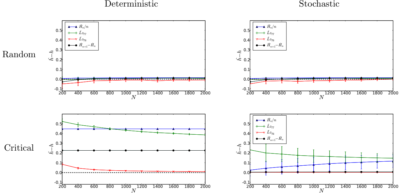
FIG. 4: Entropy estimation quality \hat{h} - h as a function of the sequence length N in the deterministic case (left column) and stochastic case (right column) for full randomness (top row) and infinite-range correlations (bottom row). Fully random sequences are generated using the chaotic logistic map with parameter a = 4 (deterministic case) and an uncorrelated Markov chain with parameter a = 1/2 (stochastic case). Sequences with infinite-range correlations are generated using the critical logistic map with parameter a = a_c \approx 3.569 (deterministic case) and Markov chain with parameter a = 10^{-3} \ll 1 i.e. with correlation time \tau(a) \approx 1/a \gg 1 (stochastic case). The entropy of 200 symbolic sequences with random initial conditions and varying length N \in [200, 2000] was computed using each estimator. Values represented on the figures correspond to the mean value over these 200 sequences. Standard deviation is depicted using vertical error bars. For the deterministic case and critical behavior, the caption inset is the same as for the other plots but for clarity, it is not depicted on the figure.
