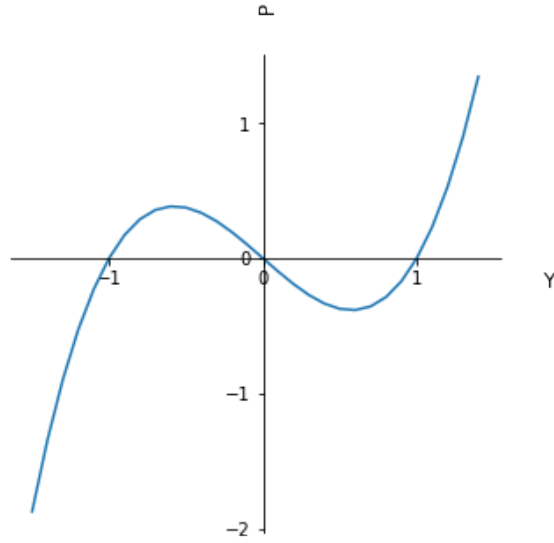
Figure 1: Plot of p = y^3 - y
