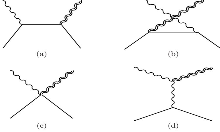
Figure 4: Diagrams relevant to graviton photo-production.
