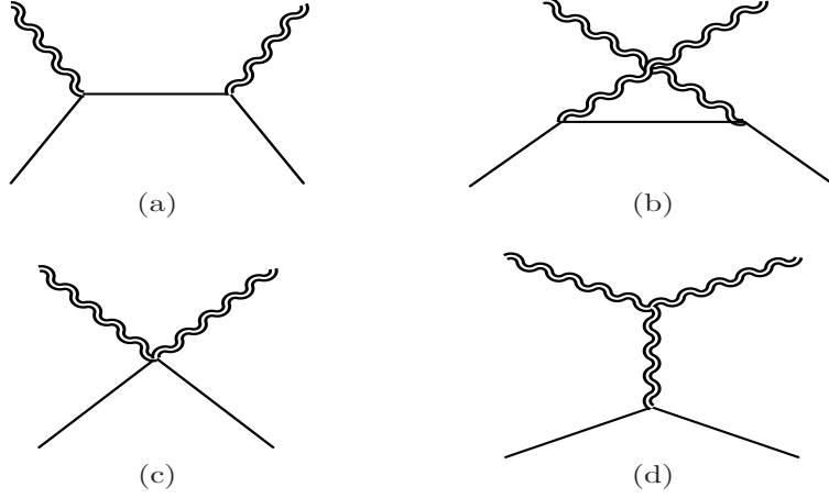
Figure 5: Diagrams relevant for gravitational Compton scattering.
