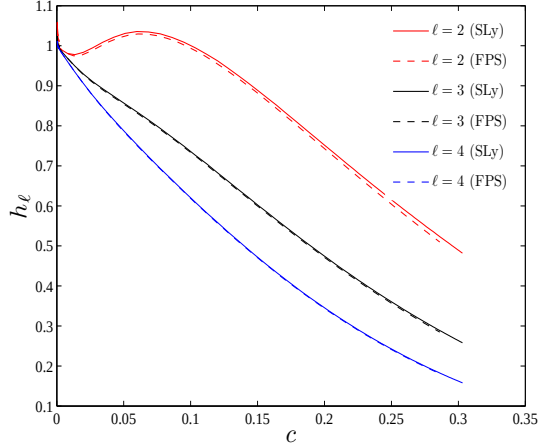
FIG. 9: Shape Love numbers h_\ell versus c for the two tabulated realistic Equation of State FPS and SLy.
