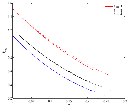
FIG. 6: Shape Love numbers h_\ell versus c for the two \gamma = 2 polytropic EOS: \mu -polytrope (solid lines) and e -polytrope (dashed lines).
