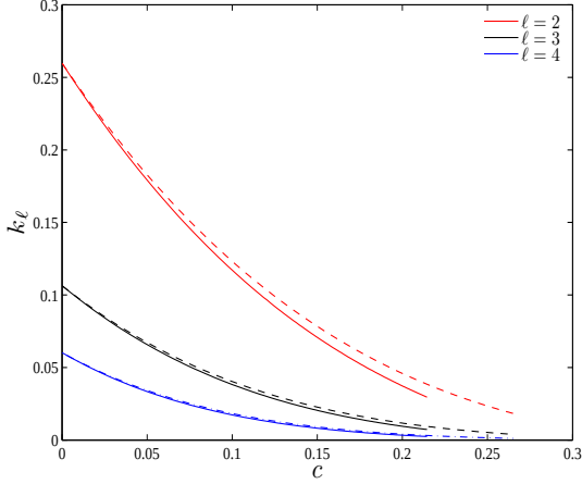
FIG. 1: Polytropic EOS: gravito-electric Love numbers k_\ell (or apsidal constants) for \ell = 2, 3, 4 versus compactness c = M/R . We use two different polytropic EOS, either of the rest-mass type ( p = \kappa\mu^\gamma ; solid lines) or of the energy type ( p = \kappa e^\gamma ; dashed lines). For both EOS we use \gamma = 2 and \kappa = 100 . Note that the maximum compactness allowed by the e -polytrope is larger than that for the \mu -polytrope.
