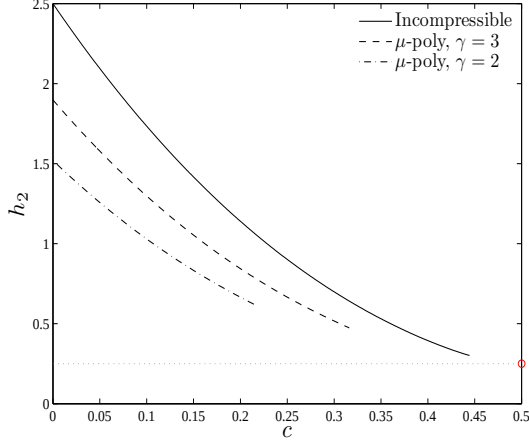
FIG. 8: Influence of the EOS on h_2(c) : comparison between the incompressible case and \mu -polytropes with two values of the polytropic index: \gamma = 2 and \gamma = 3 . The red circle on the right of the plot indicates the formal c \rightarrow 1/2 result.
