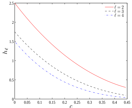
FIG. 7: Shape Love numbers h_\ell versus c for the incompressible model.
