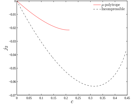
FIG. 5: The j_2 , odd-parity, Love number for the \gamma = 2 , \mu -polytrope and for the incompressible EOS.
