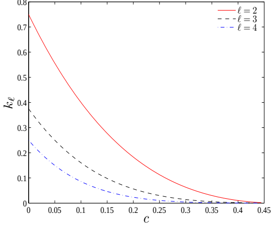
FIG. 3: Incompressible EOS: gravito-electric Love numbers k_\ell (or apsidal constants) for \ell = 2, 3, 4 versus compactness c = M/R .
