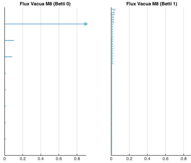
Figure 6: Barcodes for the distribution of flux vacua on X_8(1^4, 4) . The point cloud \mathbf{X} is constructed as in Figure 5. Also in this case the persistent homology computation is done using the lazy witness complex \text{LW}(\mathbf{X}, \mathbf{L}, \epsilon) , but this time the landmark set \mathbf{L} consists of 200 points randomly selected. The computation requires 852691 simplices.
