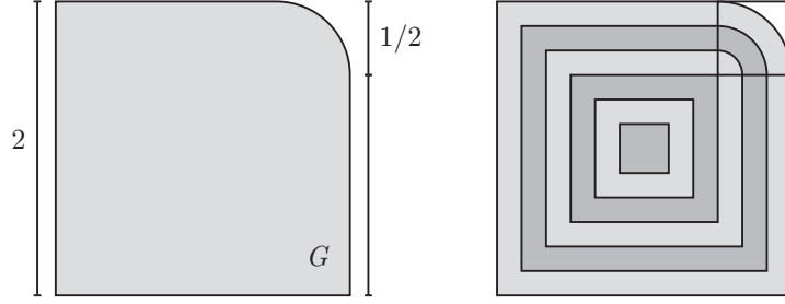
FIGURE 2. A pluriphase generator.
