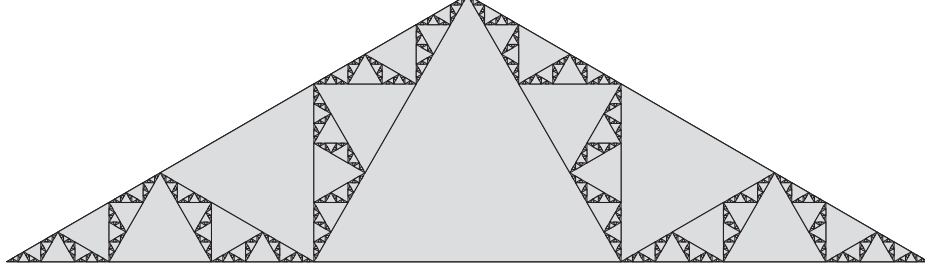
FIGURE 3. The Koch tiling \mathcal{K} .
