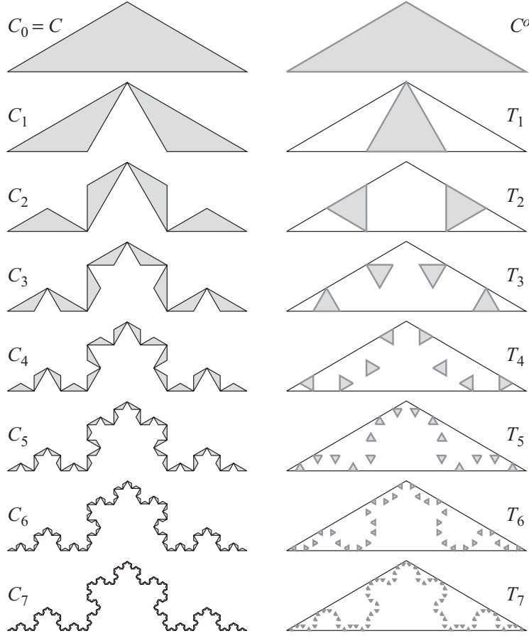
FIGURE 1. Construction of the Koch tiling \mathcal{K} . This example is discussed further in §9. The tiling \mathcal{K} has the single generator T_1 = G_1 , an equilateral triangle.
