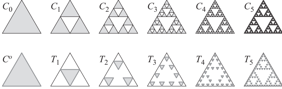
FIGURE 4. The Sierpinski gasket tiling.
