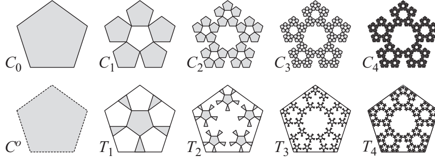
FIGURE 5. The Pentagasket tiling.
