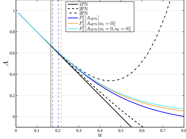
Fig. 2 Various approximations and Padé resummation of the EOB radial potential A(u) , where u = GM/(c^2 R) , for the equal-mass case v = 1/4 . The vertical dashed lines indicate the corresponding (adiabatic) LSO location [2] defined by the condition d^2 \mathcal{E}_{\text{eff}}^0 / dR^2 = d\mathcal{E}_{\text{eff}}^0 / dR = 0 , where \mathcal{E}_{\text{eff}}^0 is the effective energy along the sequence of circular orbits (i.e., when P_R^{\text{eff}} = 0 ).
