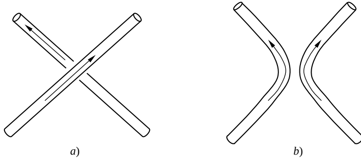
Figure 1. Shown is ‘process’ of reconnection: a) before the reconnection; b) after the reconnection.
