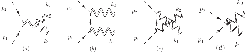
FIG. 1. The various contributions to the tree-amplitude \phi + \phi \rightarrow 2 gravitons: (a) s -channel, (b) t -channel, (c) u -channel, (d) contact term.
