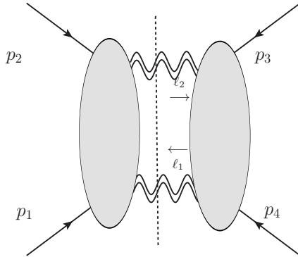
FIG. 3. The cut considered. The loop momenta are flowing clockwise. And the on-shell conditions are \ell_1^2 = 0 and \ell_2^2 = (\ell_1 + k_1 + k_2)^2 = 0 . Solid lines are massive and wiggly lines are massless.
