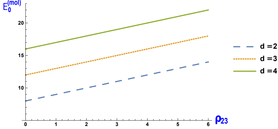
FIG. 3. Ground state energy potential curves (69) vs \rho_{23} (classical coordinate) at d = 2, 3, 4 . It corresponds to the values of the parameters a = b = m = \omega = 1 .
