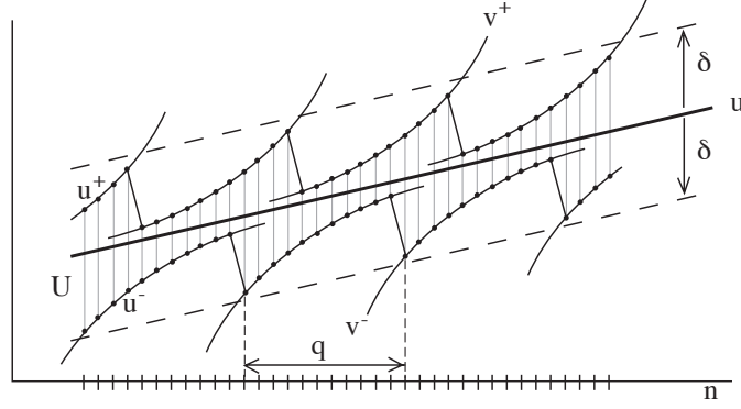
Figure 3: The neighbourhood U of \mathbf{u} bounded by \mathbf{u}^\pm , made by repeating periodically segments of length q of \mathbf{v}^\pm contained within \delta of \mathbf{u} .
