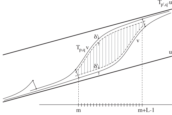
Figure 6: An “island” between \mathbf{v} and T_{pq}\mathbf{v} , avoided by states within \delta' of A_{p/q+} .
