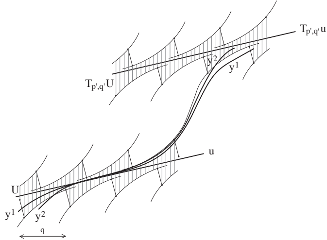
Figure 4: An Aubry diagram to show that if two segments of \mathbf{y} between entries to successive translates of U differ in length by more than q then their graphs cross.
