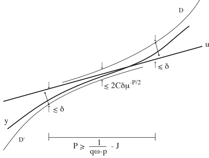
Figure 8: Halfway between entry and exit of \mathbf{y} in/out of U , the chosen discommensurations \mathbf{D} , \mathbf{D}' are within C\delta\mu^{-P/2} of \mathbf{u} , with P \geq \frac{1}{q\omega-p} - J .
