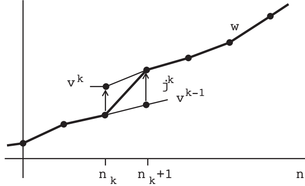
Figure 1: An Aubry diagram showing the jump from state \mathbf{v}^{k-1} to \mathbf{v}^k at n = n_k .
