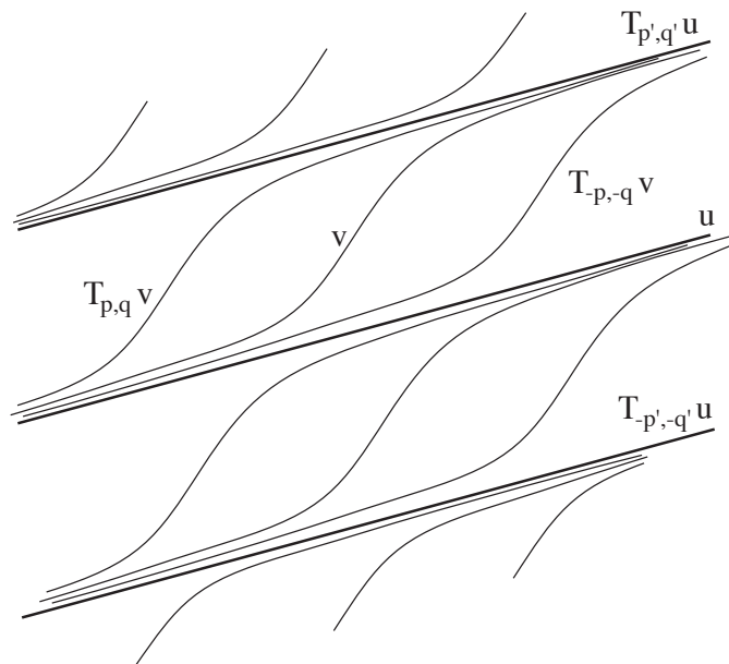
Figure 2: An Aubry diagram illustrating that the states in A'_{p/q+} form a lamination of the plane (to simplify, we draw the graphs of \mathbf{u} and its translates as straight lines and of \mathbf{v} and its translates as smooth curves, rather than piecewise affine).
