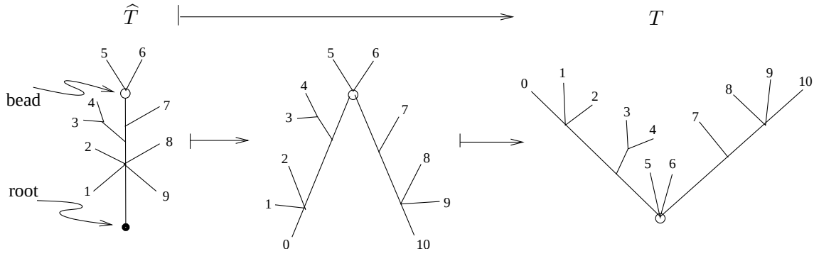
FIGURE 1. A \Psi -tree obtained from a fan
