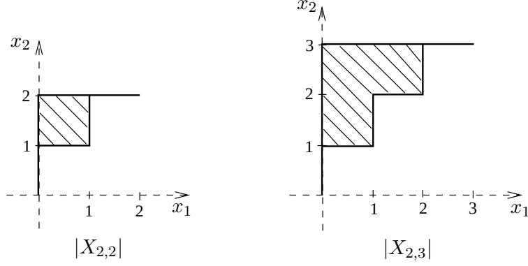
FIGURE 3. Examples of |X_{\ell,r}| .
