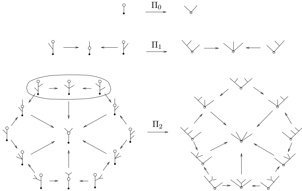
FIGURE 2. \Pi_0 , \Pi_1 , \Pi_2 . The circled edge of the hexagon gets mapped to the top vertex of the pentagon.
