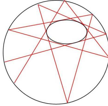
Figure 4: Poncelet configuration
