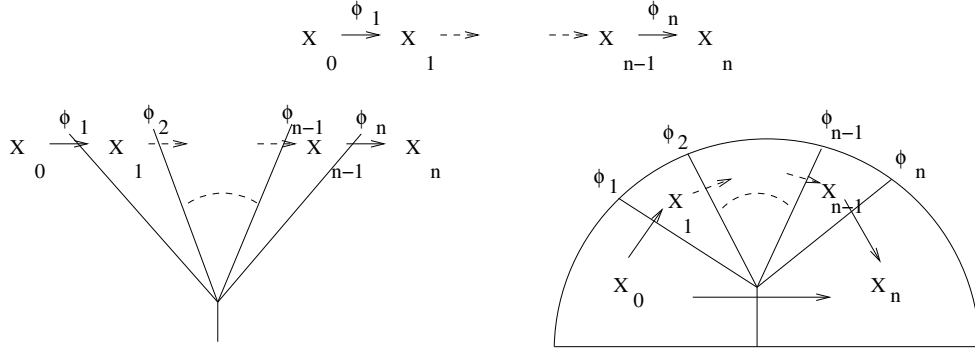
FIGURE 13. Marking a corolla by a simplex in N_*(\mathcal{C}) . The morphisms decorate the ends of the tree, while the objects decorate the angles which correspond to the marks on the half circle
