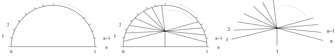
FIGURE 10. The interval injection [1] \rightarrow [n] on the left, the surjection \underline{n} \rightarrow \underline{1} on the right and Joyal duality in the middle. Here reading the morphism upwards yields the double base point preserving injection, while reading it downward the surjection.
