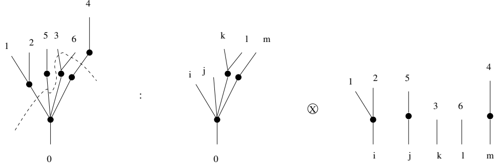
FIGURE 4. One term of the coproduct corresponding to the indicated cut in the labelled case.
