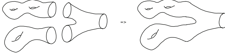
FIGURE 2. Fusion
