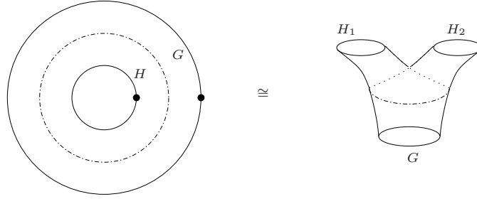
FIGURE 3. Fission
