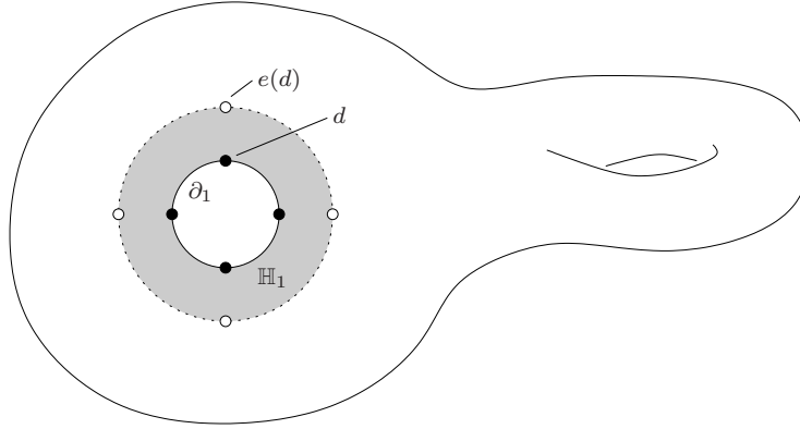
FIGURE 1. The surface \tilde{\Sigma} with halo drawn
